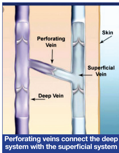
Figure 1: The superficial and deep venous system of the lower leg.
